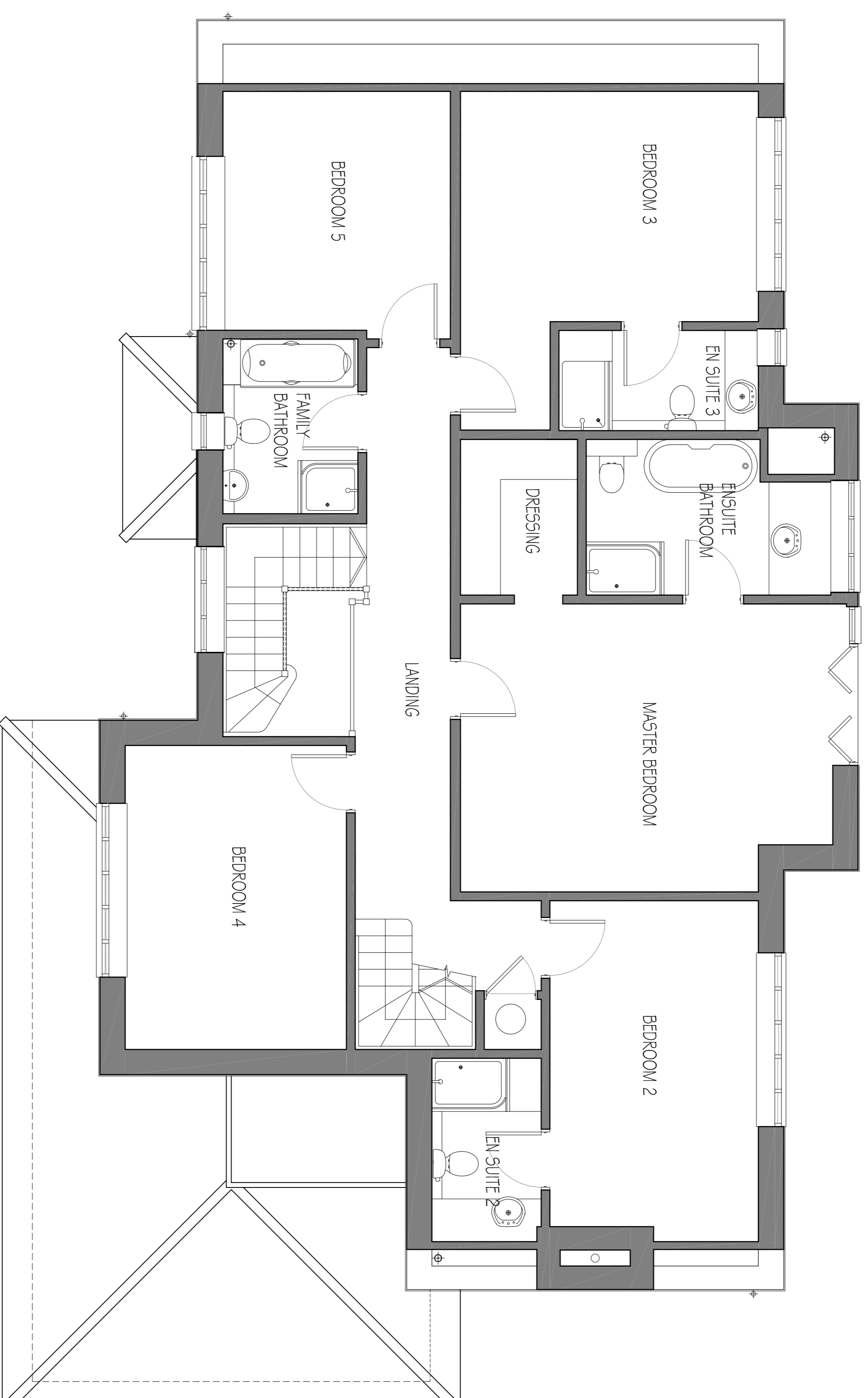
PROPOSED FIRST FLOOR PLAN - PLOT 1 PL REF: 17-082 SCALE: 1:50 (A1), 1:100 (A3)
