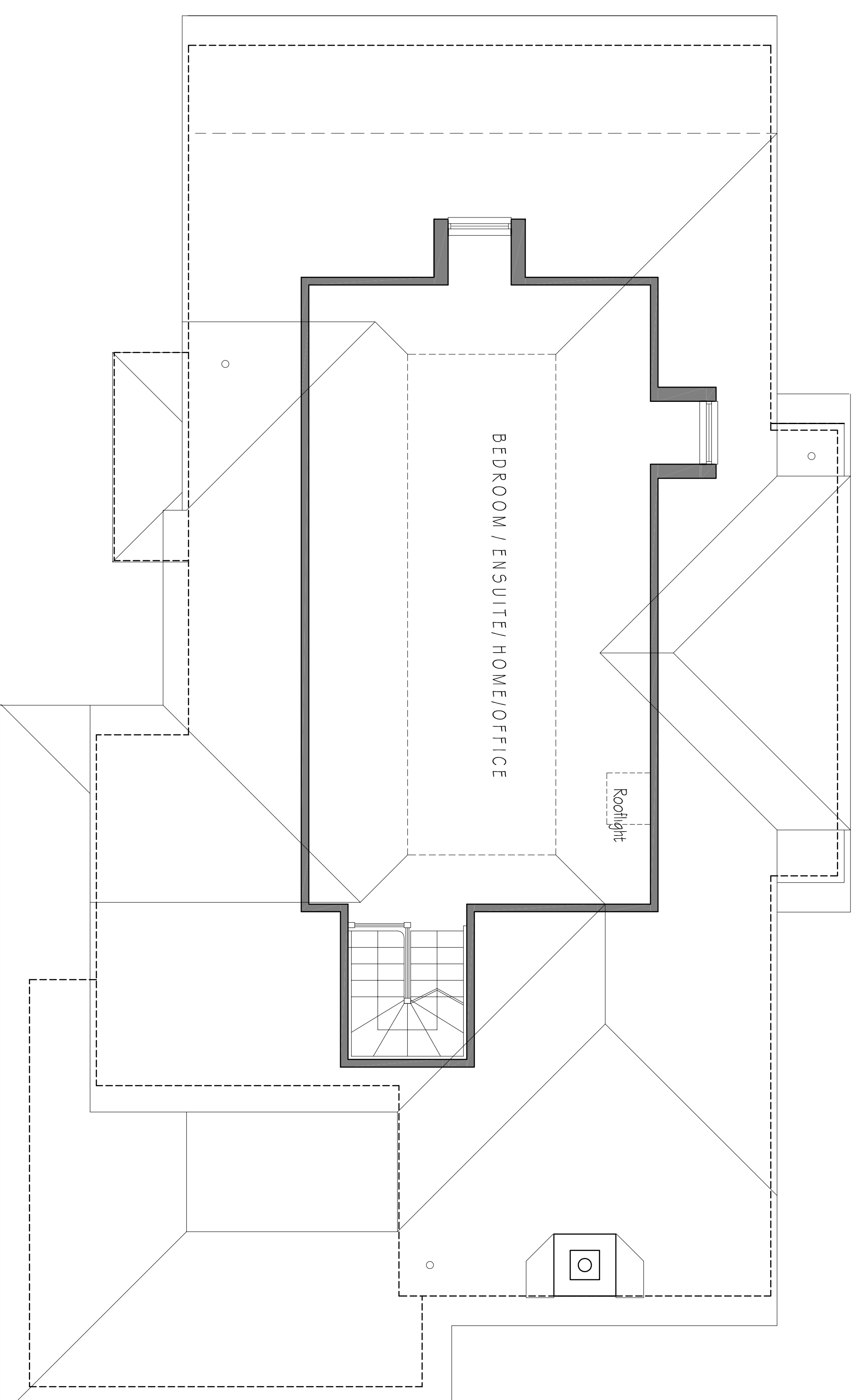
PL PROPOSED SECOND FLOOR PLAN - PLOT 1 REF: 17-082 SCALE: 1:50 (A1), 1:100 (A3)
